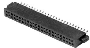
Part Nos. Available CFS-50-A-SG-SMT-A (No offset) CFS-50-A-SG-SMT-B (0.3mm offset) CFS-50-A-SG-SMT-C (0.6mm offset) CFS-50-A-SG-SMT-D (0.9mm offset)
