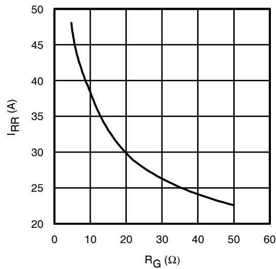
Fig. 20 - Typ. Diode I_{RR} vs. R_G T_J = 175^\circ C
