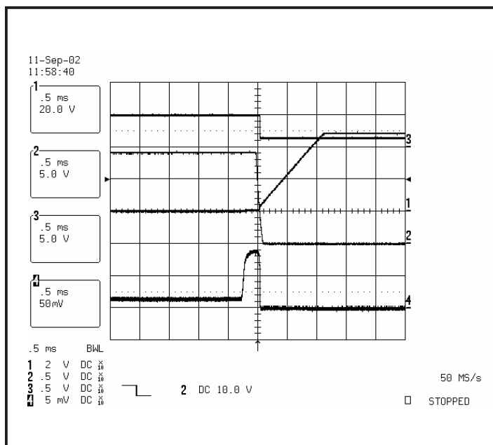
Figure 6. Over-current/Short circuit.
