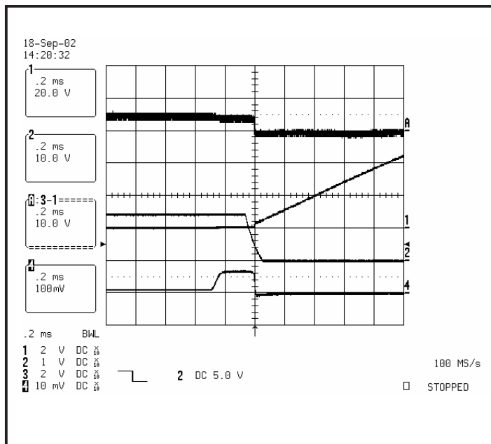
Figure 10. Over-current/Short circuit.
