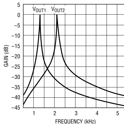
Frequency Response
