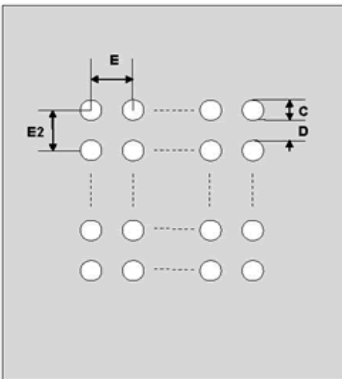
Top View (SMT Footprint)
