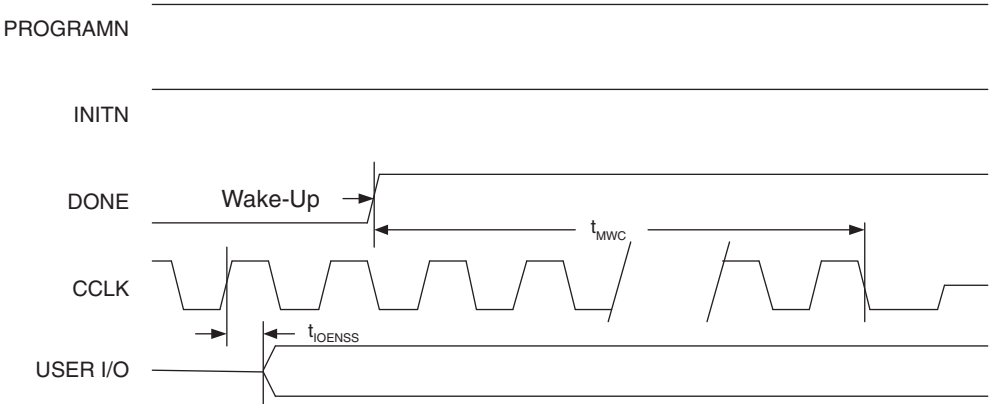
Figure 3-23. Wake-Up Timing
