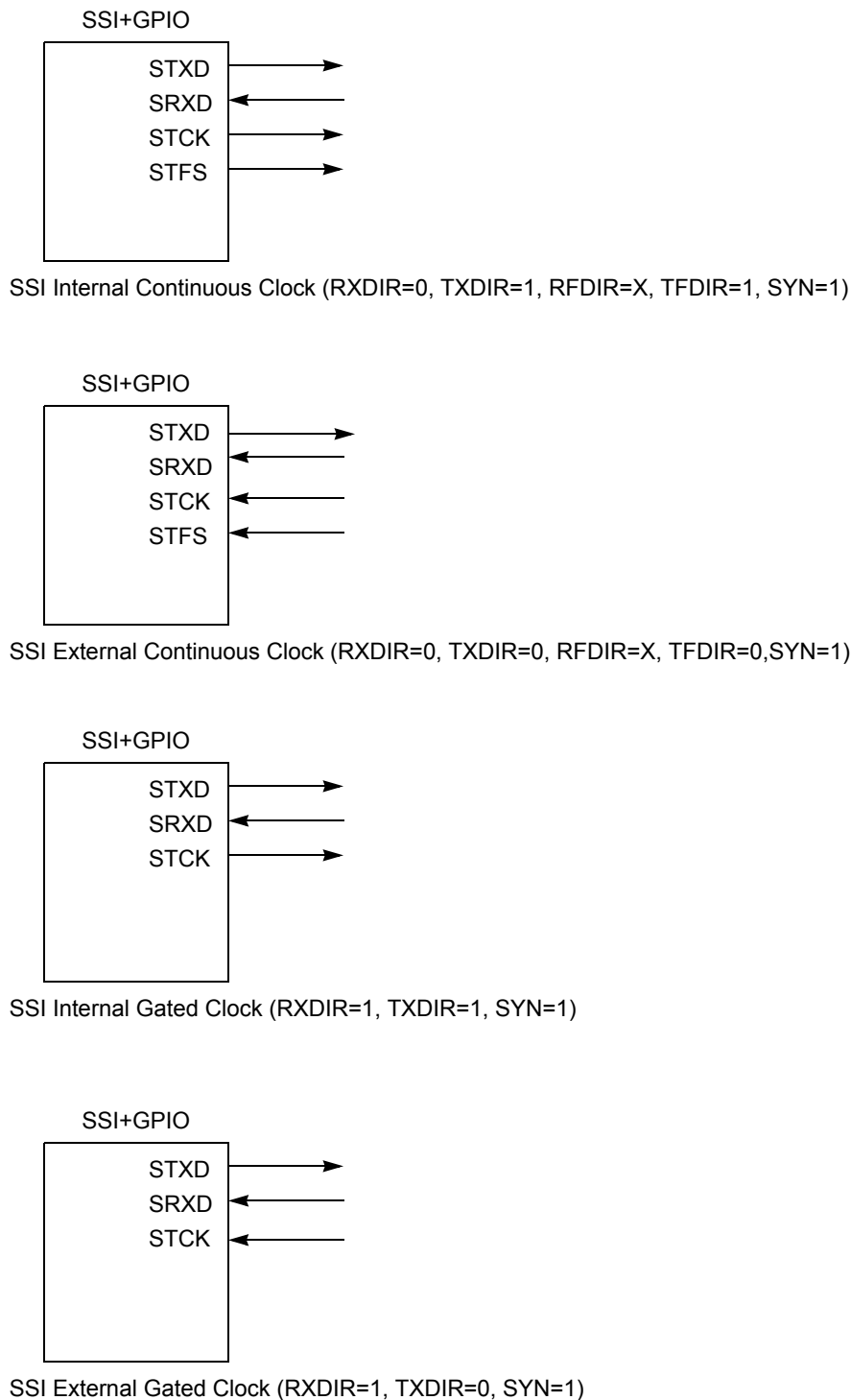
Figure 50. Synchronous SSI Configurations—Continuous and Gated Clock
