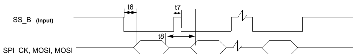
Figure 48. Slave CSPI Timing FIFO Advanced by SS_B Rising Edge
