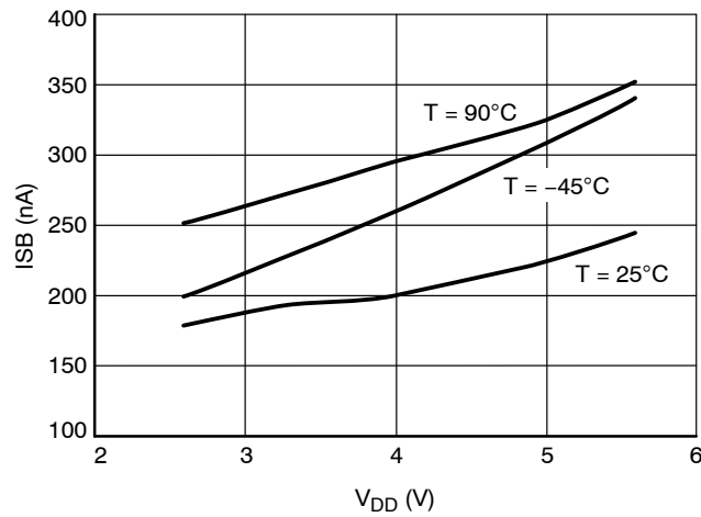
Figure 9. Standby Current
