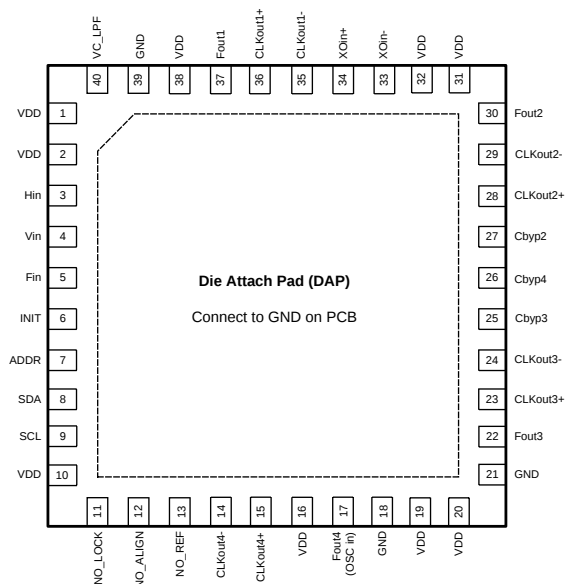
Pin Functions
