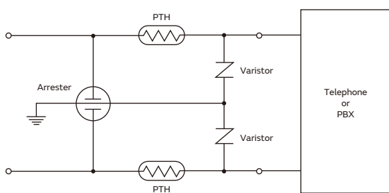
(5) Telecommunication Circuit
