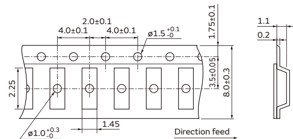
PR*21_RA Series: Embossed Tape
