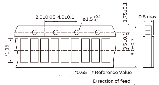
PR*21_RA Series: Embossed Tape
