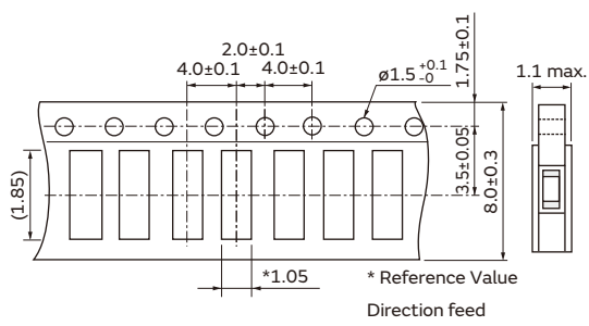
PRG21_RK Series: Embossed Tape
