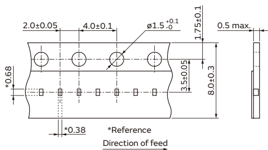
PR*18_RB Series: Paper Tape
