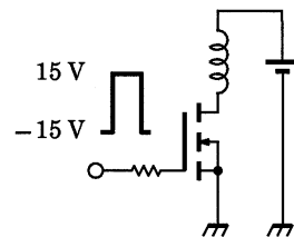
TEST CIRCUIT
