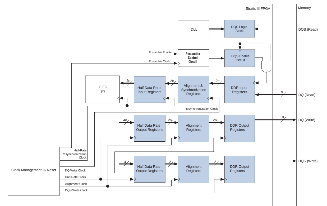
Figure 8–2. External Memory Interface Data Path Overview (Note 1), (2), (3)
