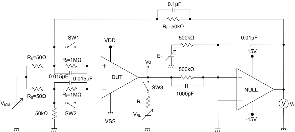
Figure 24. Test Circuit 1
