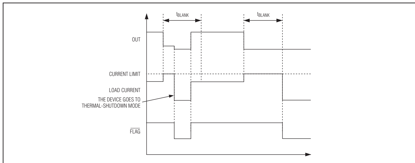
Figure 3. Latchoff Fault Diagram
