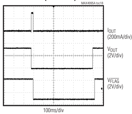
FLAG RESPONSE (OVERLOAD) CONDITION
