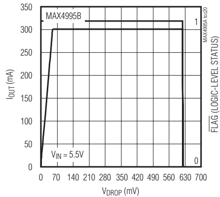
I_{OUT}/FLAG vs. V_{DROP} ( V_{IN} - V_{OUT} )
