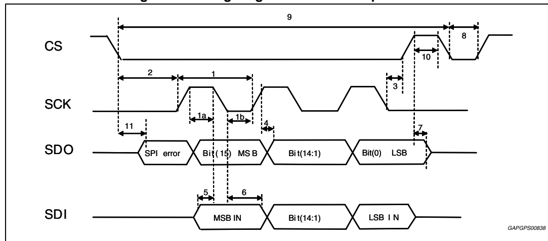
Figure 7. Timing diagram for the SPI operation.
