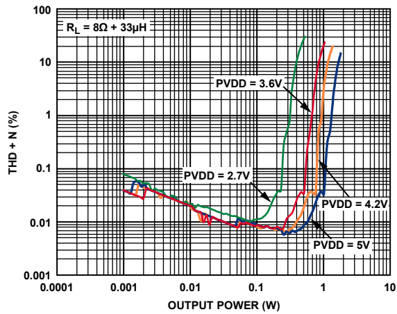
Figure 4. THD + N vs. Output Power into 8 \Omega , Class-D Amplifier, Mono Operation
