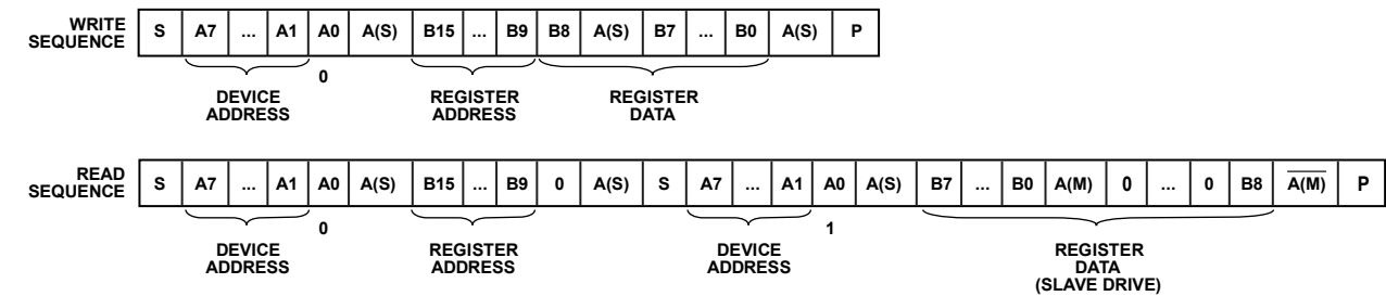
Figure 37. 2-Wire I 2 C Generalized Clocking Diagram
