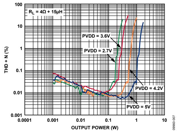
Figure 8. THD + N vs. Output Power into 4 \Omega , Class-D Amplifier, Stereo Operation
