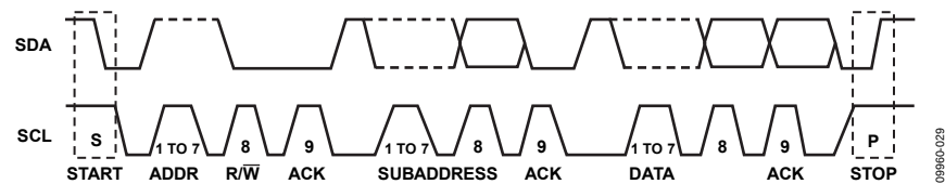
Figure 37. 2-Wire I 2 C Generalized Clocking Diagram
