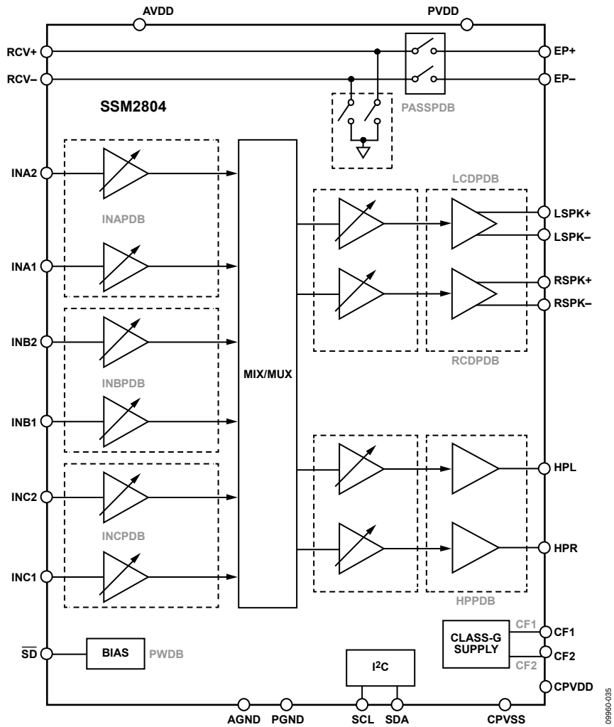
Figure 39. Power Management Control Register Blocks
