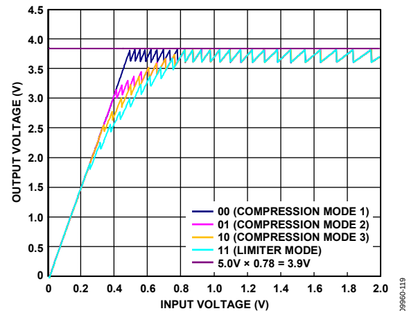
Figure 33. Adjustable Compression Settings, PVDD = 5.0 V, ALC Threshold Level = 78%
