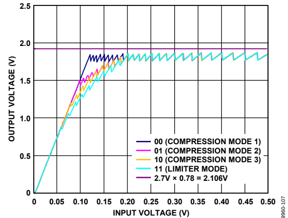
Figure 31. Adjustable Compression Settings, PVDD = 2.7 V, ALC Threshold Level = 78%
