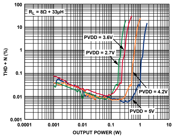
Figure 5. THD + N vs. Output Power into 8 \Omega , Class-D Amplifier, Stereo Operation
