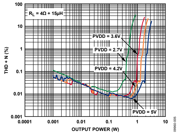
Figure 7. THD + N vs. Output Power into 4 \Omega , Class-D Amplifier, Mono Operation
