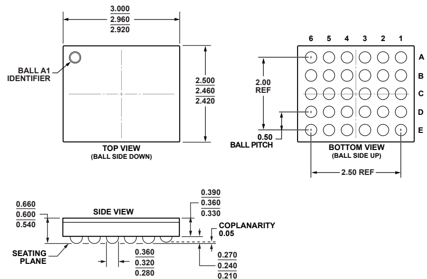
Figure 40. 30-Ball Wafer Level Chip Scale Package [WLCSP] (CB-30-4) Dimensions shown in millimeters
