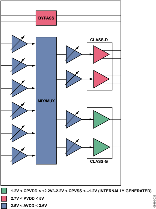
Figure 36. Power Supply Domains
