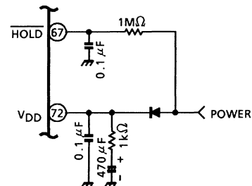
Example of a Condenser Back-Up Circuit
