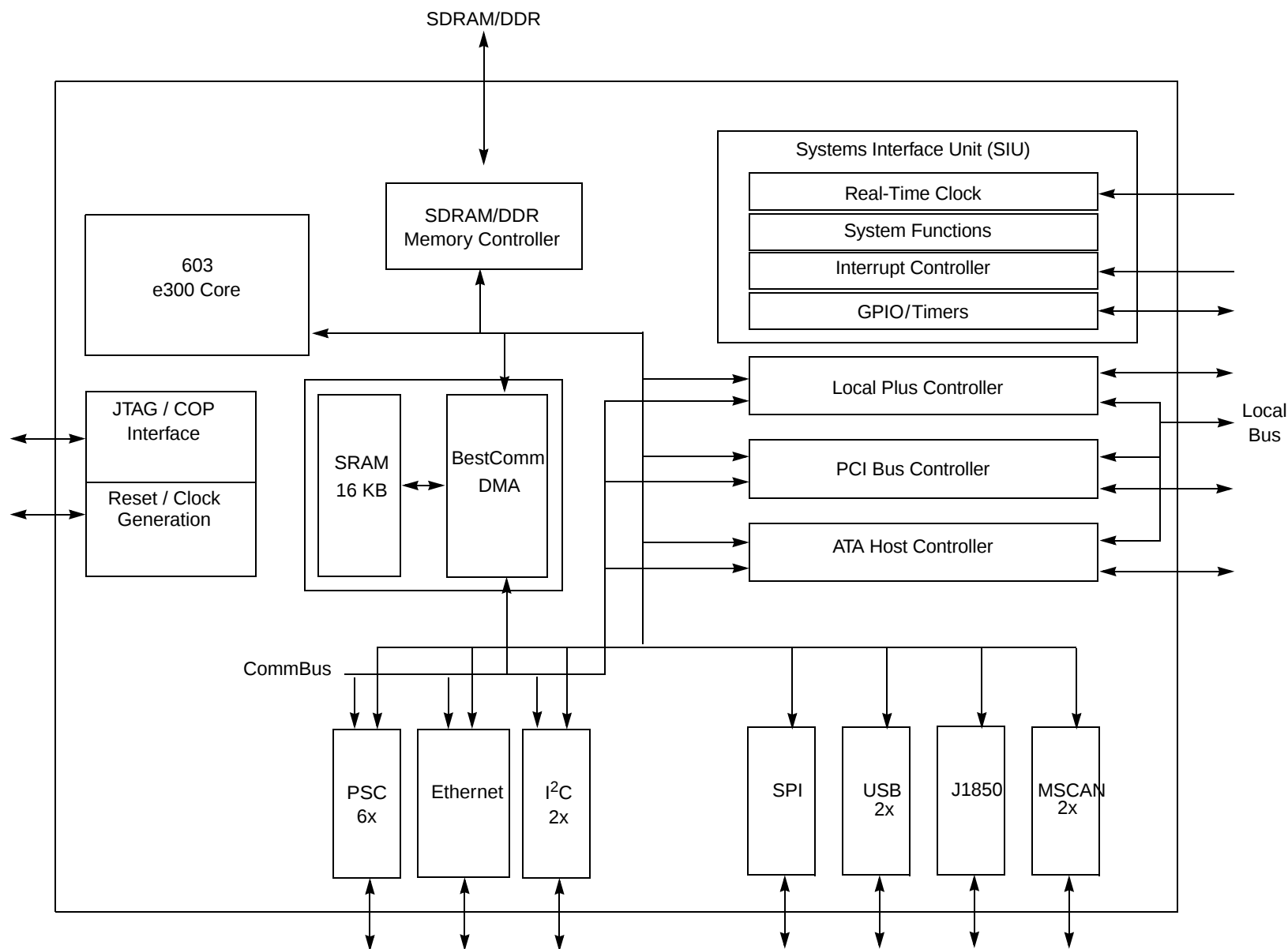
Figure 1. Simplified Block Diagram—MPC5200B
