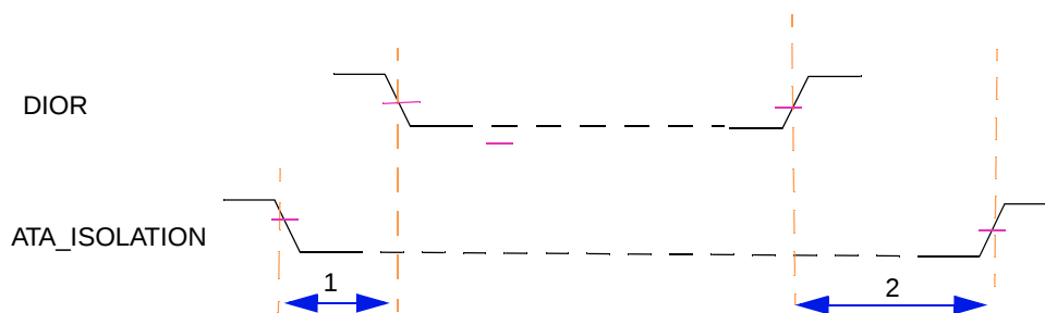
Figure 26. Timing Diagram—ATA-ISOLATION
