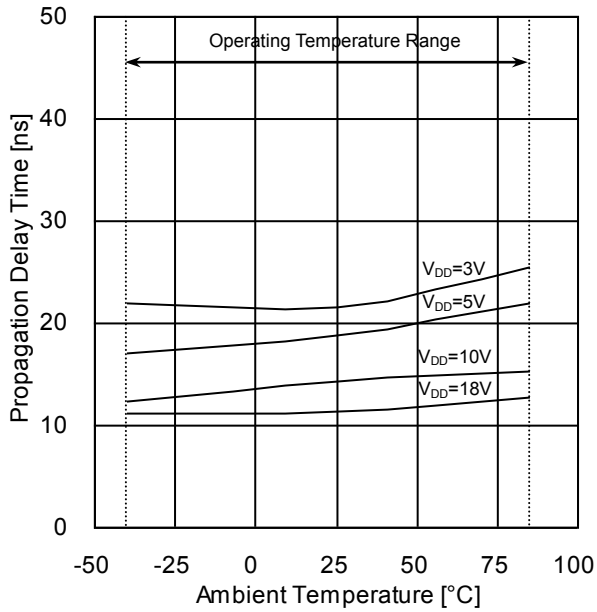
Figure 11. Propagation Delay Time IN→OUT( t_{PLH} ) vs Ambient Temperature
