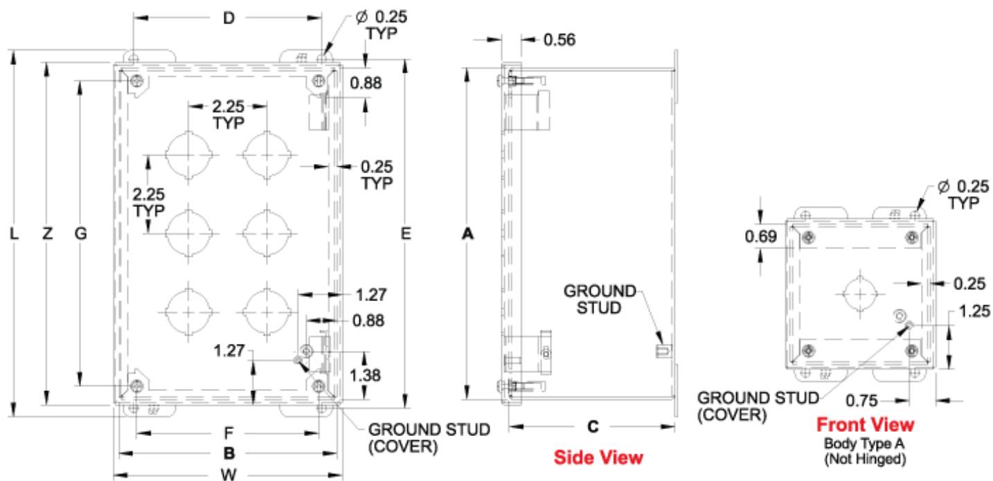
Front View Body Type B through X (Hinged)
