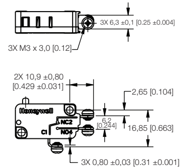
Figure 13. V15 Series T-style Screw Terminal
