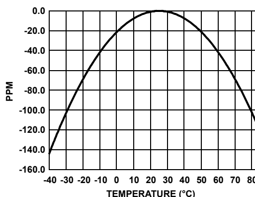
FIGURE 18. RTC CRYSTAL TEMPERATURE DRIFT
