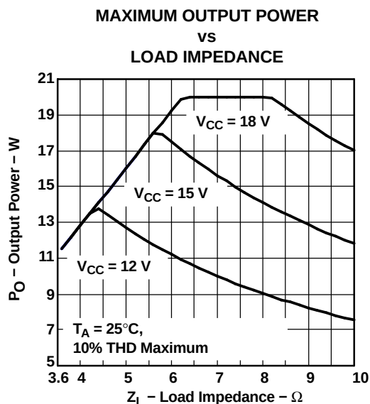
Figure 23. Output Power
