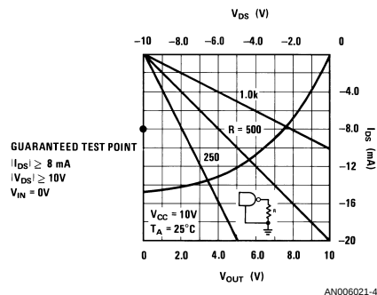
(B) Typical Output Source Characteristic (P-Channel)
