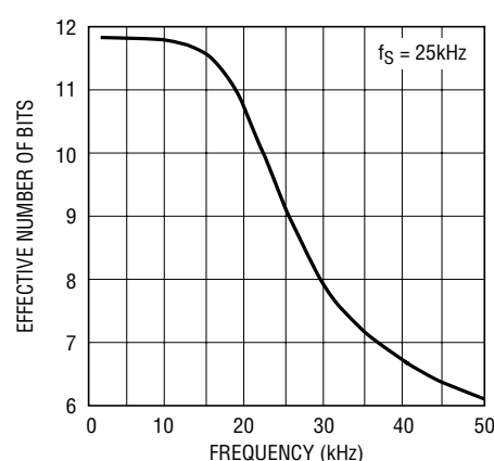
LTC1289 • A1F18
