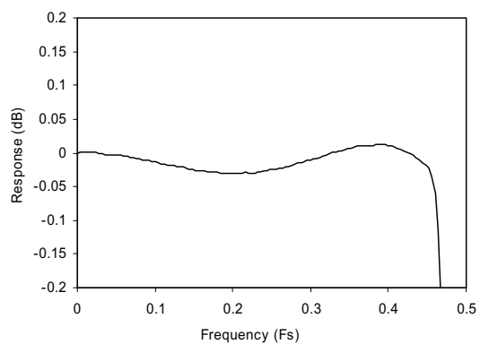
Figure 29 DAC Digital Filter Ripple
