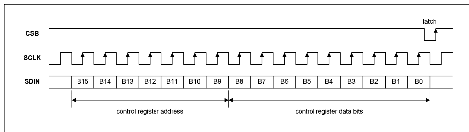
Figure 26 3-Wire Serial Control Interface
