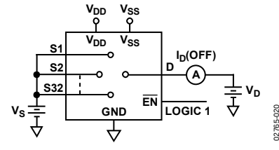
Figure 24. I_D (Off)
