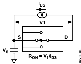
Figure 20. On Resistance
