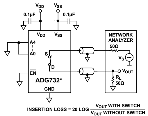
Figure 26. Bandwidth
