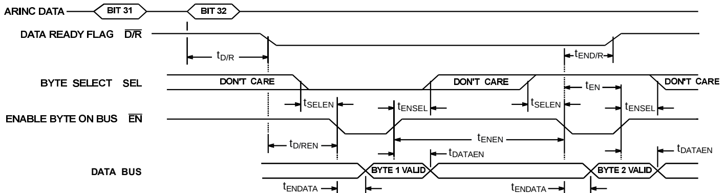
RECEIVER OPERATION
