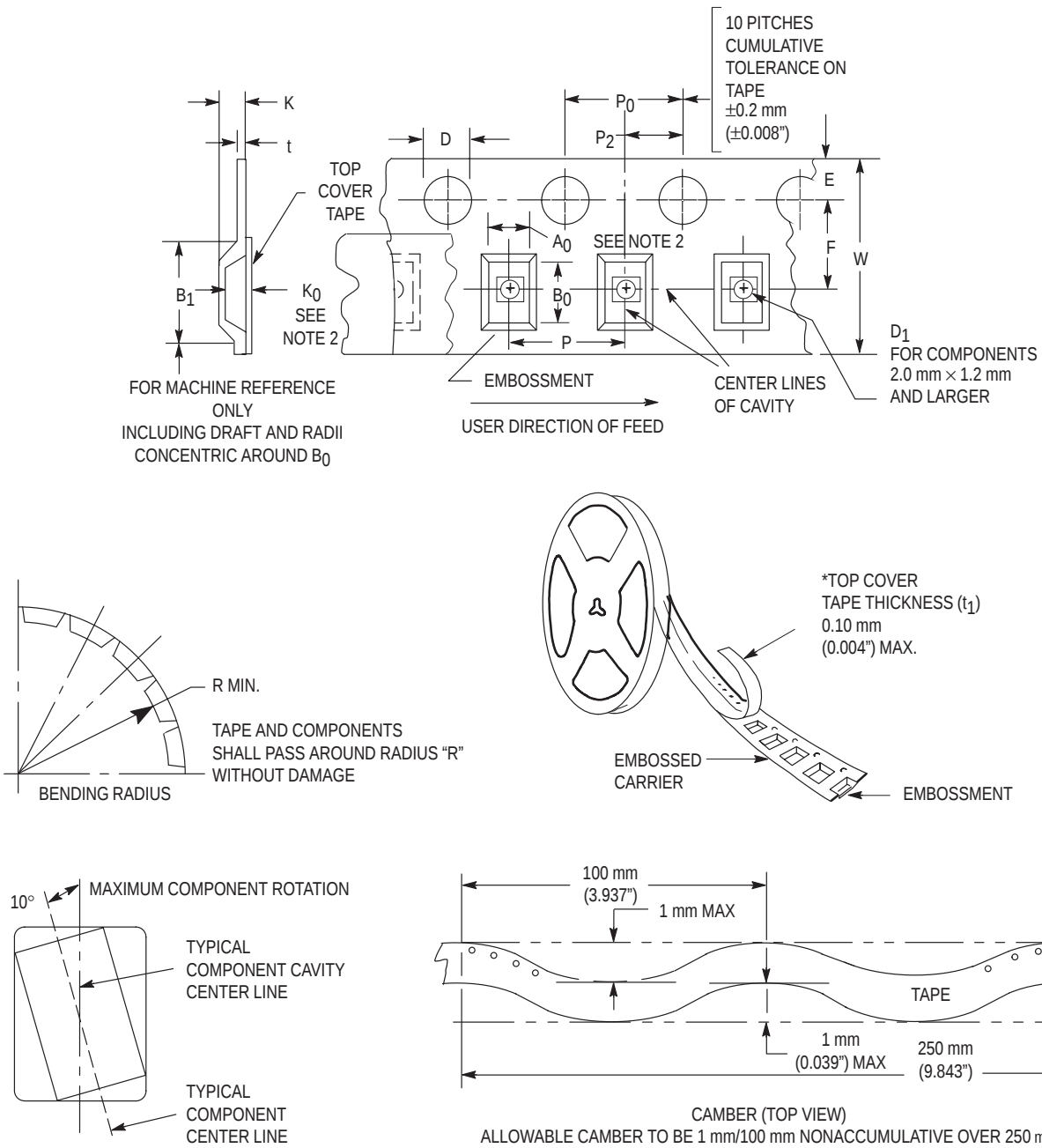
Figure 4. Carrier Tape Specifications
