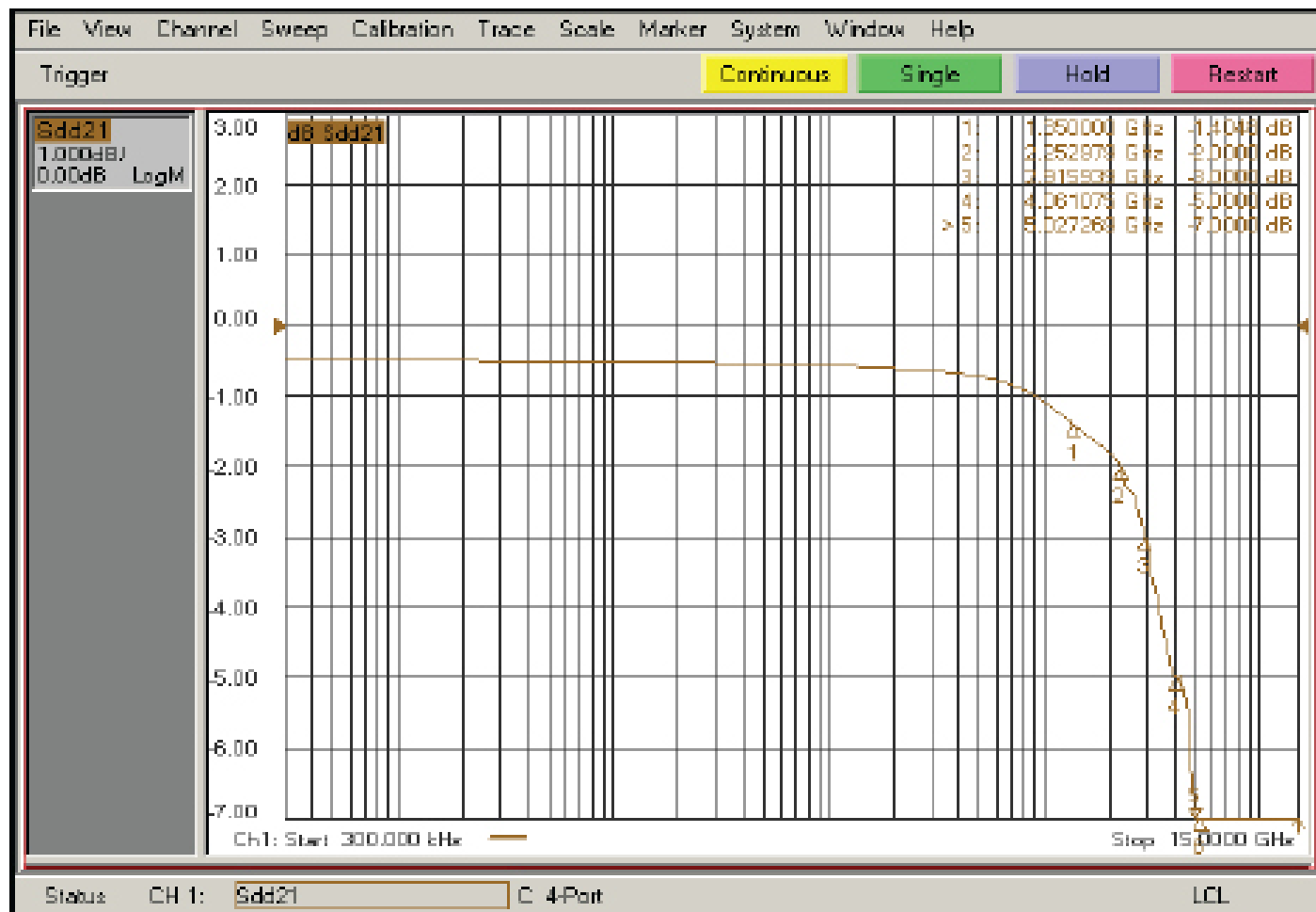
Fig 6. Insertion Loss
