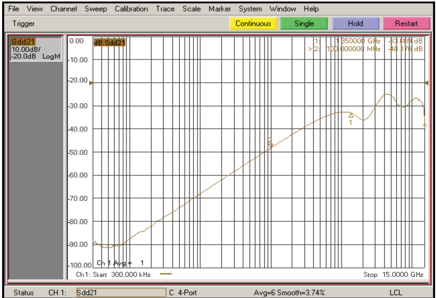
Fig 4. Crosstalk
