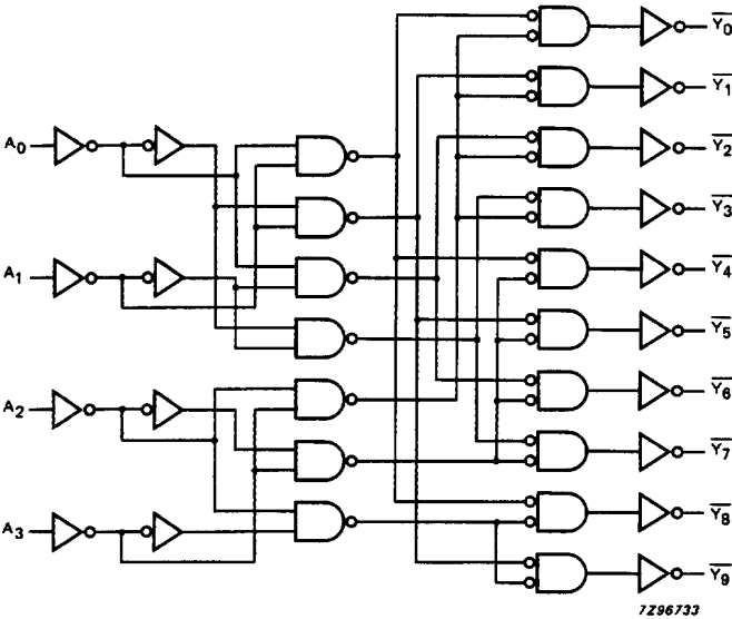
Fig.5 Logic diagram.
