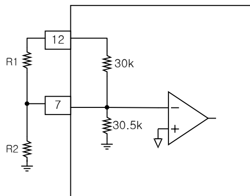
Figure 2. Output Voltage
