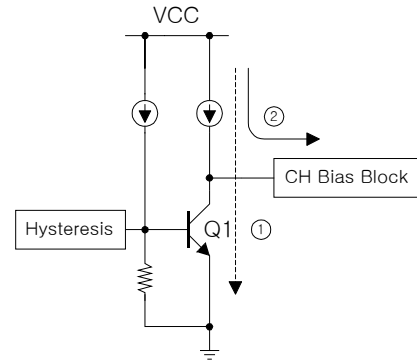
Figure 2. TSD Circuit
