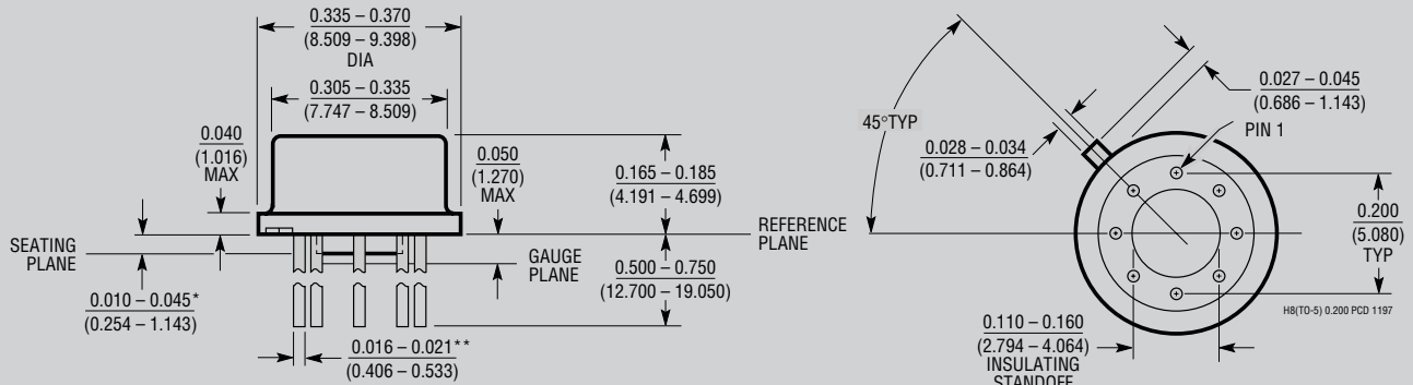
H Package 8-Lead TO-5 Metal Can (.200 Inch PCD) (Reference LTC DWG # 05-08-1320)
