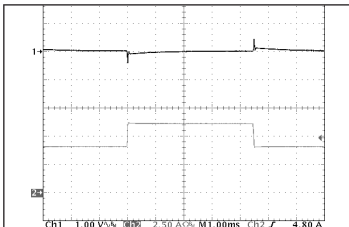
Figure 5: Output voltage response to step-change in load current (50%-75%-50% of Iout(max); dI/dt = 0.1A/μs). Load cap: 15μF tantalum cap and 1μF ceramic cap. Ch 1: Vout (1V/div), Ch 2: Iout (2.5A/div).
