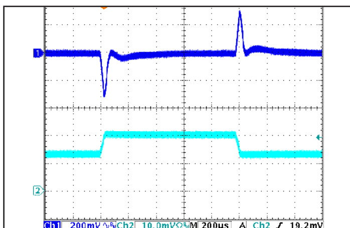
Figure 5: Output voltage response to step-change in load current (50%-75%-50% of I out (max); dI/dt = 0.1A/μs). Load cap: 15μF tantalum cap and 1μF ceramic cap. Ch 1: V out (200mV/div), Ch 2: I out (5A/div).
