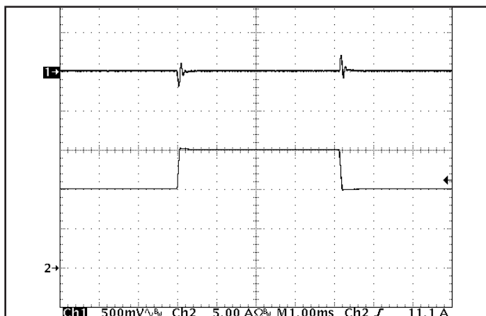
Figure 5: Output voltage response to step-change in load current (50%-75%-50% of I out (max); dI/dt = 0.1A/μs). Load cap: 15μF tantalum cap and 1μF ceramic cap. Ch 1: V out (500mV/div), Ch 2: I out (5A/div).
