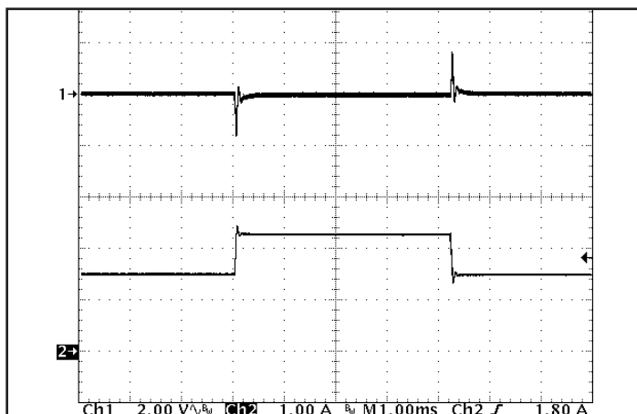
Figure 5: Output voltage response to step-change in load current (50%-75%-50% of Iout(max); dI/dt = 0.05A/μs). Load cap: 1μF ceramic cap. Ch 1: Vout (2V/div), Ch 2: Iout (1A/div).
