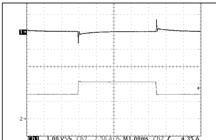
Figure 5: Output voltage response to step-change in load current (50%-75%-50% of I out (max); dI/dt = 0.1A/μs). Load cap: 15μF tantalum cap and 1μF ceramic cap. Ch 1: V out (1V/div), Ch 2: I out (2.5A/div).
