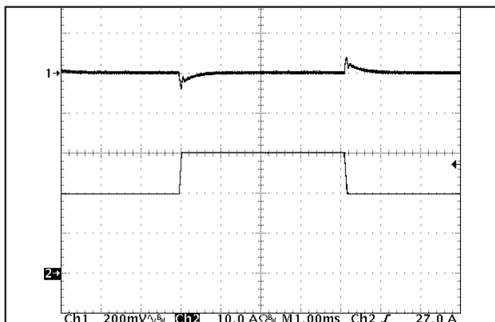
Figure 5: Output voltage response to step-change in load current (50%-75%-50% of I out (max); dI/dt = 0.2A/μs). Load cap: 1μF ceramic cap and 15μF tantalum cap. Ch 1: V out (200mV/div), Ch 2: I out (10A/div).
