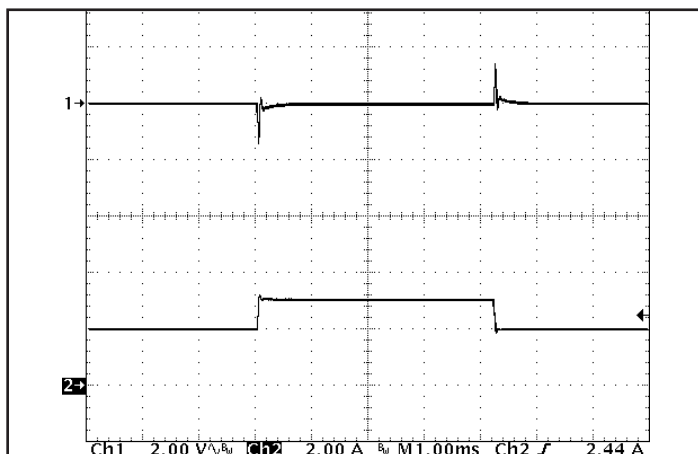
Figure 5: Output voltage response to step-change in load current (50%-75%-50% of Iout(max); dI/dt = 0.08A/μs). Load cap: 1μF ceramic cap. Ch 1: Vout (2V/div), Ch 2: Iout (2A/div).
