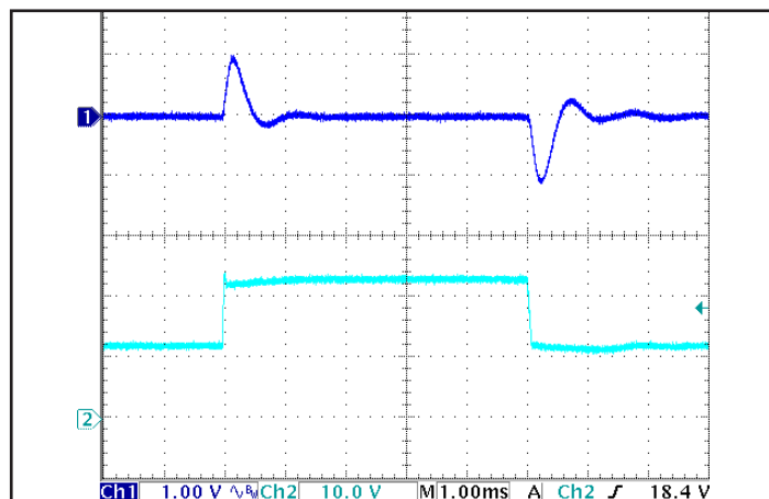
Figure 6: Output voltage response to step-change in input voltage (nominal to maximum, 250 V/ms). Load cap: 1μF ceramic capacitor. Ch 1: Vout, Ch 2: Vin.
