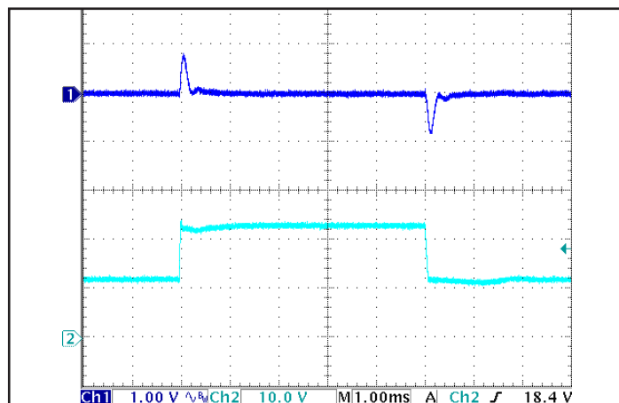
Figure 6: Output voltage response to step-change in input voltage (250V/ms). Load cap: 100μF electrolytic output capacitance. Ch 1: Vout (1V/div), Ch 2: Vin (10V/div).
