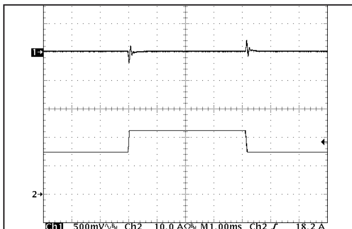
Figure 5: Output voltage response to step-change in load current (50%-75%-50% of I out (max); dI/dt = 0.2A/μs). Load cap: 15μF tantalum cap and 1μF ceramic cap. Ch 1: V out (500mV/div), Ch 2: I out (10A/div).
