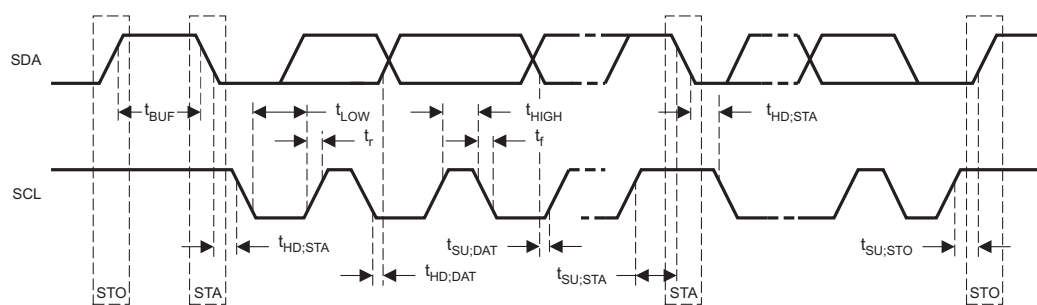
Figure 5-5. I²C Interface Timing Diagram
