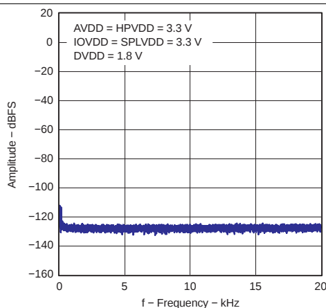
Figure 5-6. FFT – ADC Idle Channel Differential
