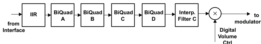
Figure 7-25. Signal Chain for PRB_P19 and PRB_P22
