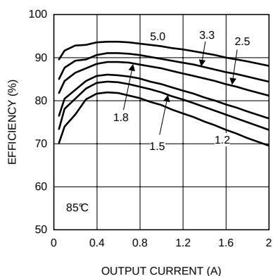
Figure 19. Efficiency 8-V Input at 85°C
