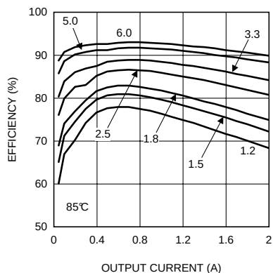
Figure 21. Efficiency 12-V Input at 85°C
