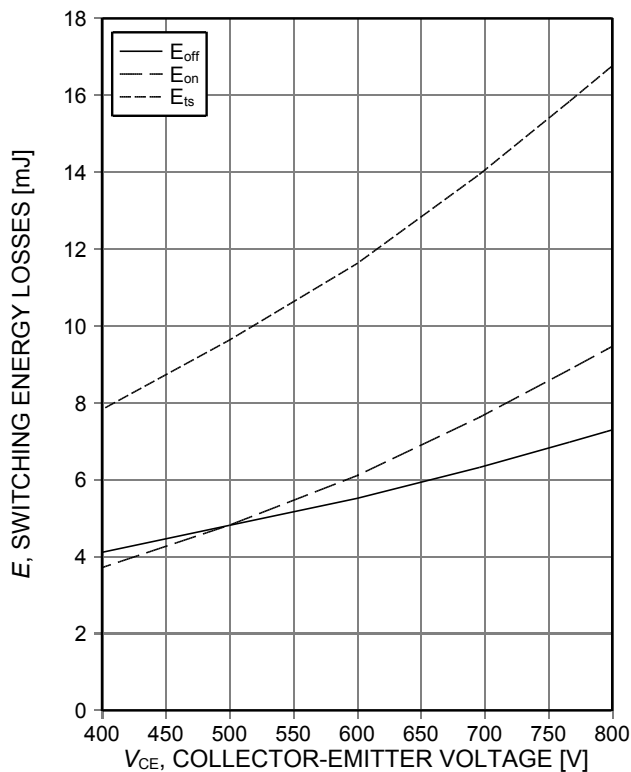
Figure 15. Typical switching energy losses as a function of collector emitter voltage (inductive load, T_{vj}=175^\circ\text{C} , V_{GE}=15/0\text{V} , I_C=50\text{A} , r_G=10\Omega , Dynamic test circuit in Figure E)
