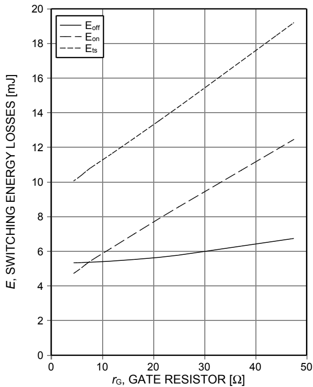
Figure 13. Typical switching energy losses as a function of gate resistor (inductive load, T_{vj}=175^\circ\text{C} , V_{CE}=600\text{V} , V_{GE}=15/0\text{V} , I_C=50\text{A} , Dynamic test circuit in Figure E)
