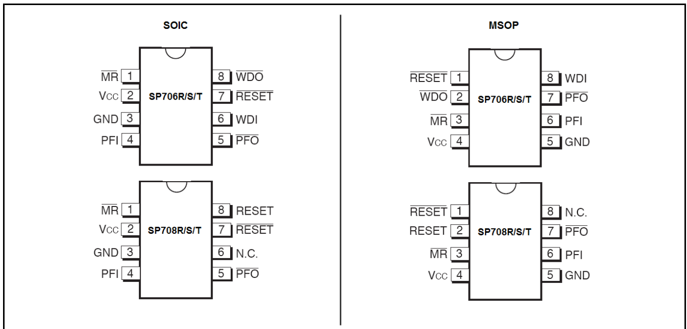
Fig. 3: Pin Assignment
