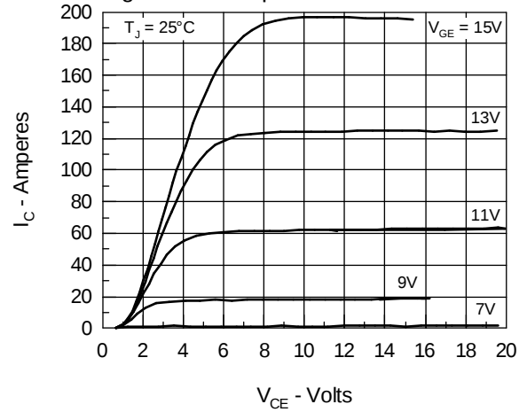
Fig. 2 Output Characteristics
