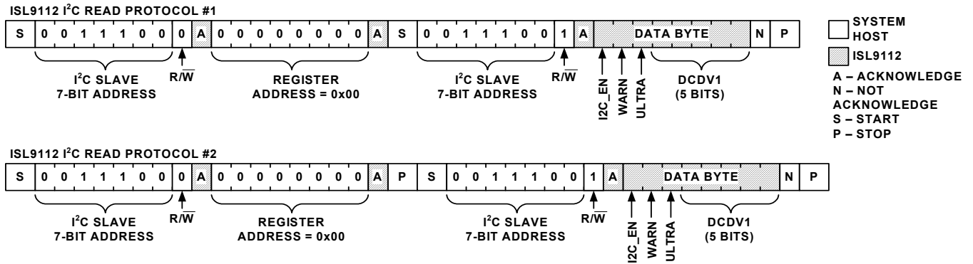
FIGURE 31. I²C REGISTER READ PROTOCOL
