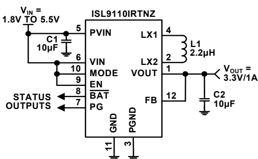
FIGURE 1. TYPICAL APPLICATION
