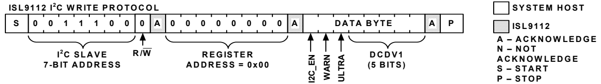
FIGURE 30. I²C REGISTER WRITE PROTOCOL
