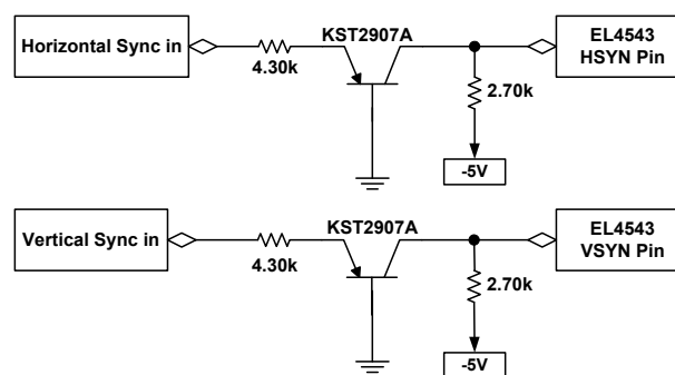
FIGURE 40. LEVEL SHIFTING SYNC SIGNALS FOR USE WITH \pm 5\text{V} SPLIT RAILS
