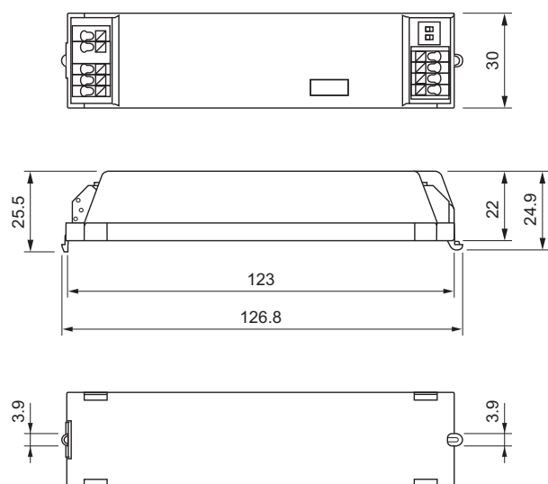
LLC1655/00 Actilume 1-10V Switchbox
