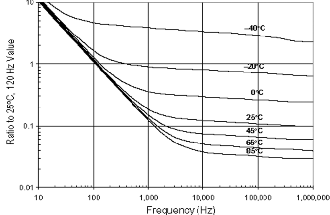
Impedance vs. Temperature and Frequency
