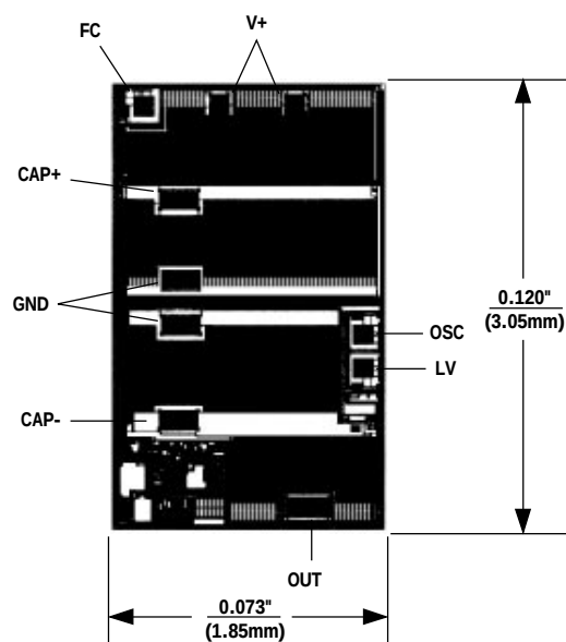
Chip Topography
