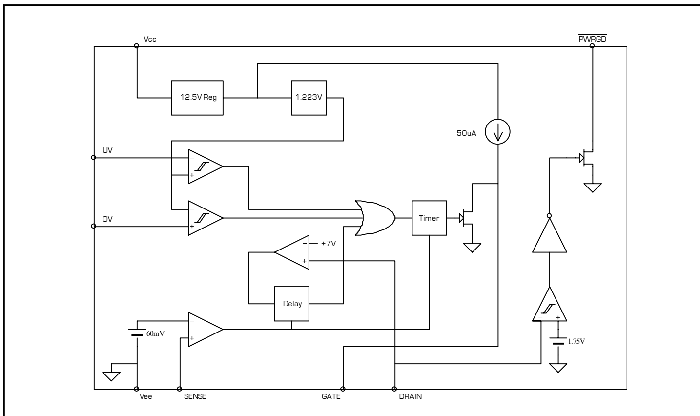
Active Low \overline{\text{PWRGD}}
