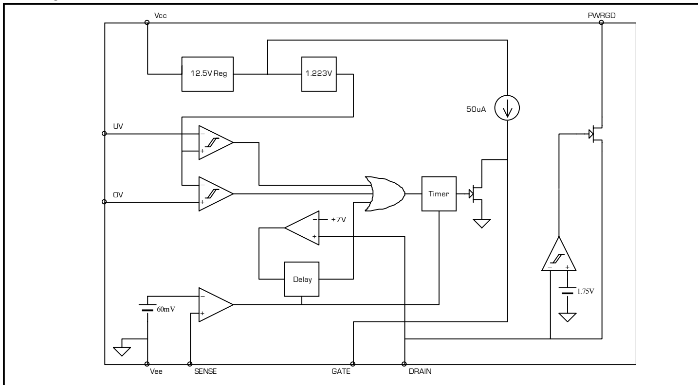
Active High PWRGD
