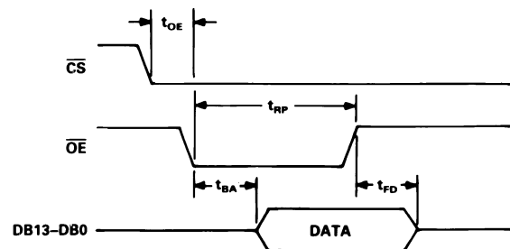
Figure 3. EOC Timing
