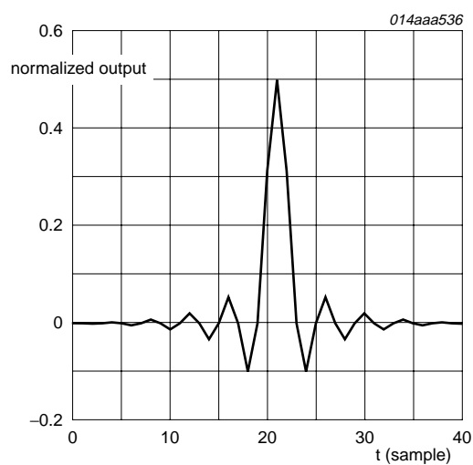
Fig 7. FIR filter impulse response
