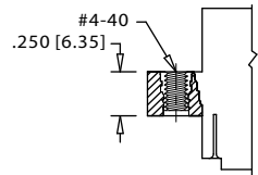
THREADED INSERT (T)
