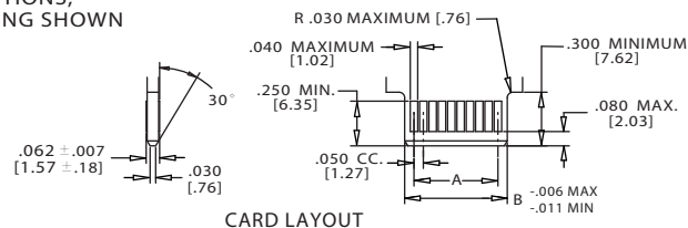
CARD LAYOUT
