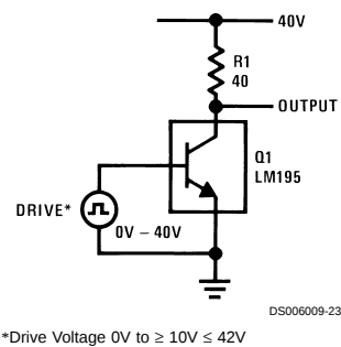
40V Switch
