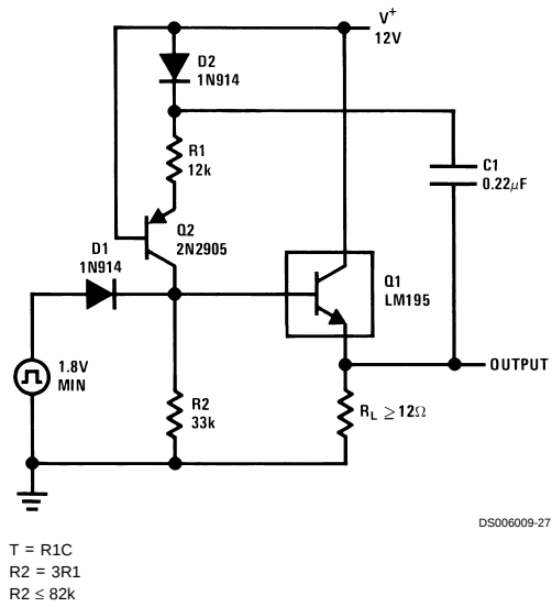
Power One-Shot
