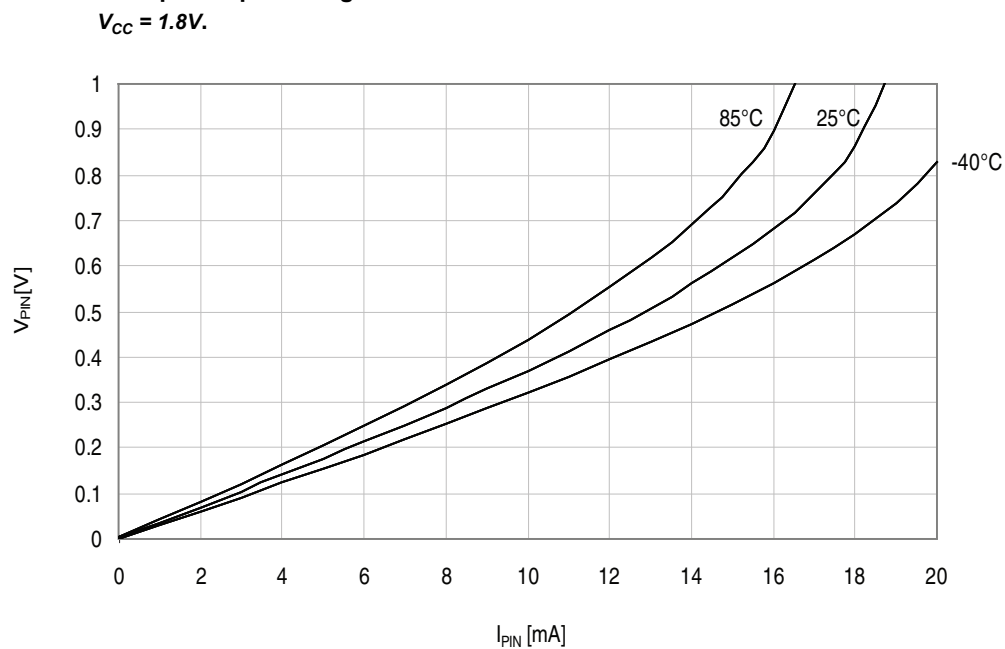
Figure 33-268. I/O pin output voltage vs. sink current.
